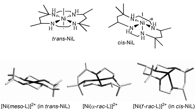
Figure 1. The structures of [Ni( meso -L)] 2+ , [Ni( α - rac -L)] 2+ and [Ni( f - rac -L)] 2+ .
